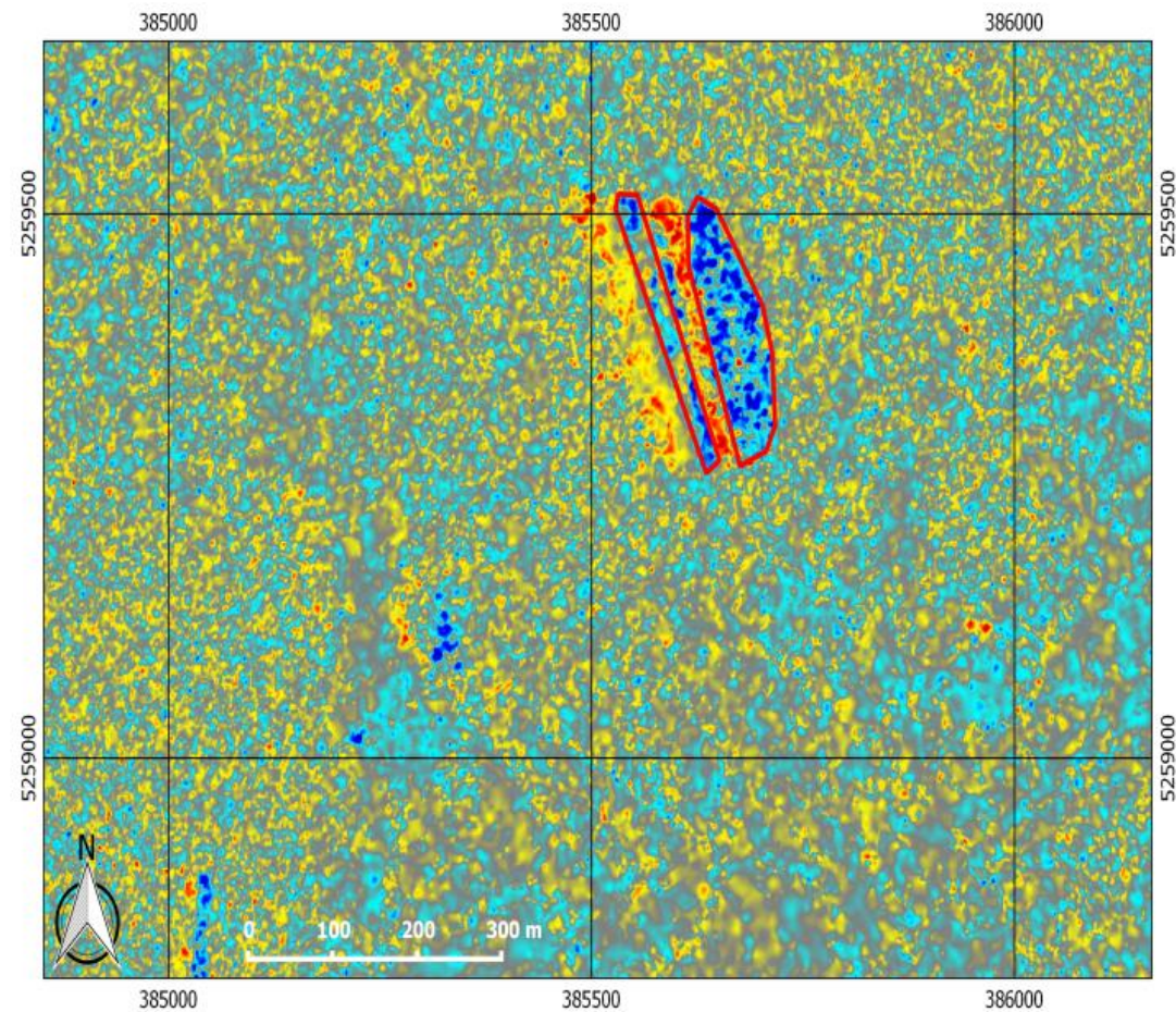
Fast detection of forest damage caused by severe storms (2 ha) as seen by satellite radar
